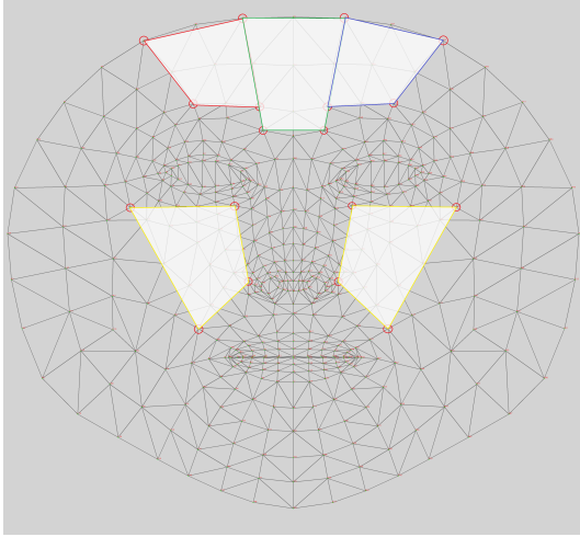
Fig. 3. Face landmarks that are created by the Mediapipe Face Mesh program, and extracted ROIs. The areas with red, green, and blue outlines represent the right, center and left forehead, and the areas with yellow outlines represent the right and left cheek.
